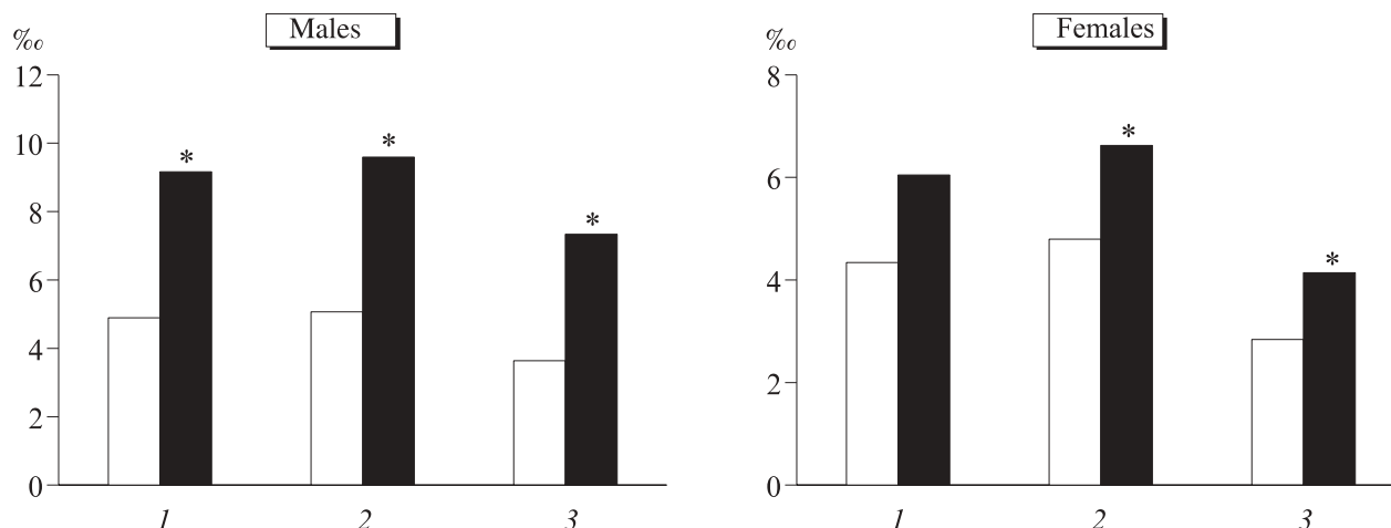
Fig. 1. Effect of intrauterine hypoxia on mitotic index of the myocardium in newborn rats: left ventricle (1), interventricular septum (2), and right ventricle (3). Light bars: control. Dark bars: treatment. * p < 0.05 compared to the control.
